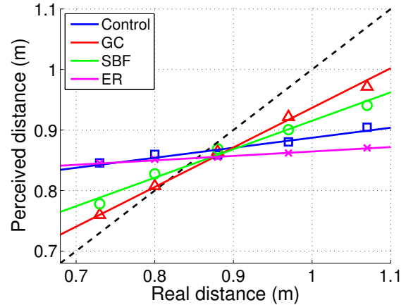
Figure 4: Perceived distances as a function of rendered distance for each sonification condition. «□, △, ○, ×»: Mean under each condition. Lines: Mean of linear regression.
