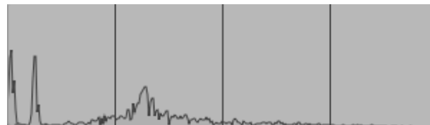
Figure 5: Spectrogram showing fundamental, sub-harmonic and higher frequency noise components of the resulting tone.
